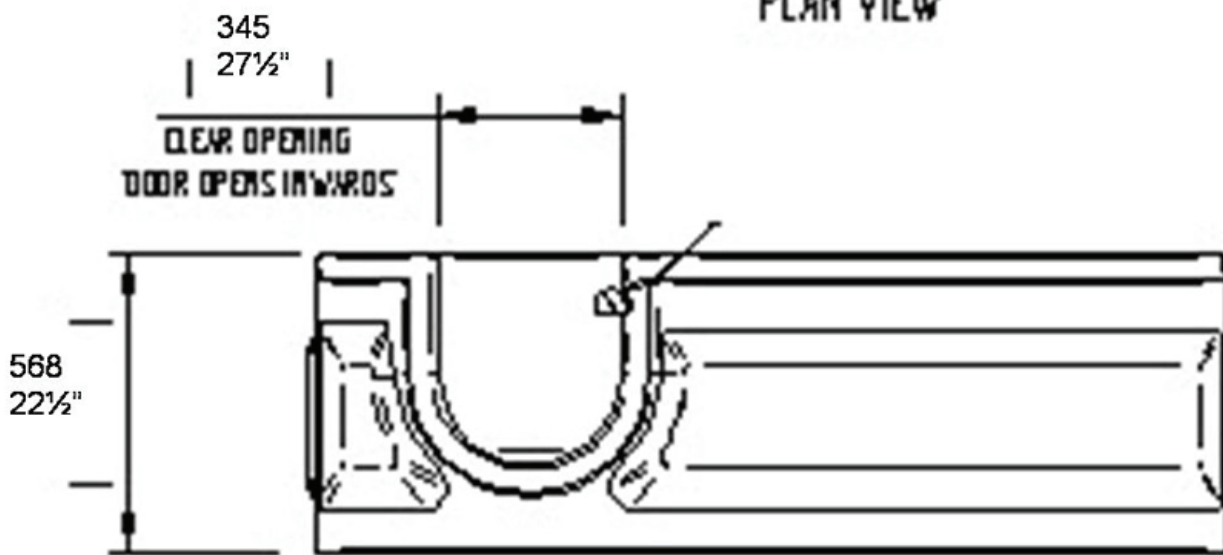
FRONT ELEVATION
