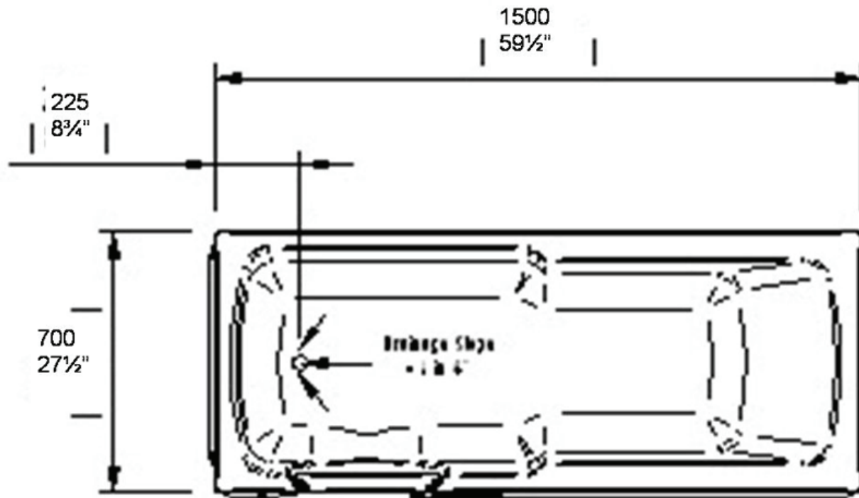
PLAN VIEW
